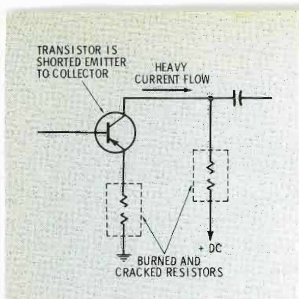
Fig. 1 Simply replacing obviously defective parts will not always solve the real problem. Here, the shorted transistor will only burn out replacement resistors.
