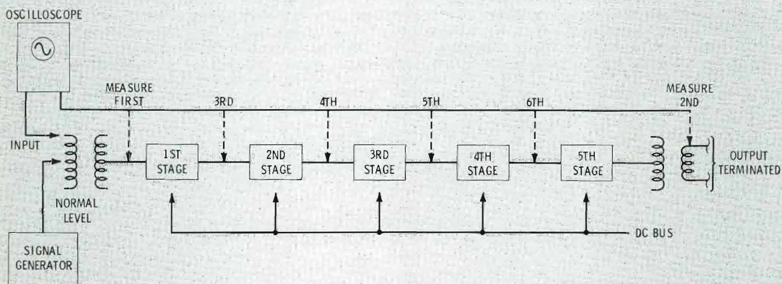
Fig. 2 Signal tracing is a fast isolation technique. First measure the input and output signals, then proceed from stage to stage until signal fails.
