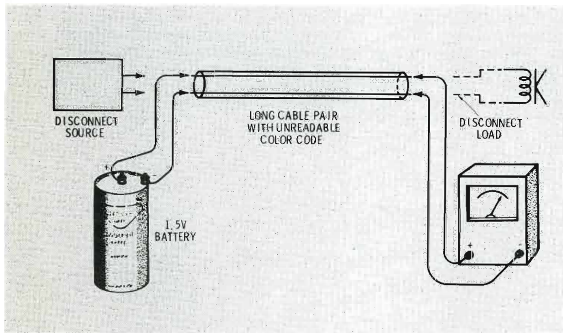
Fig. 6 You can make use of a dry cell battery and a DC voltmeter to check the phasing of a cable pair when the color code is undeadable.
